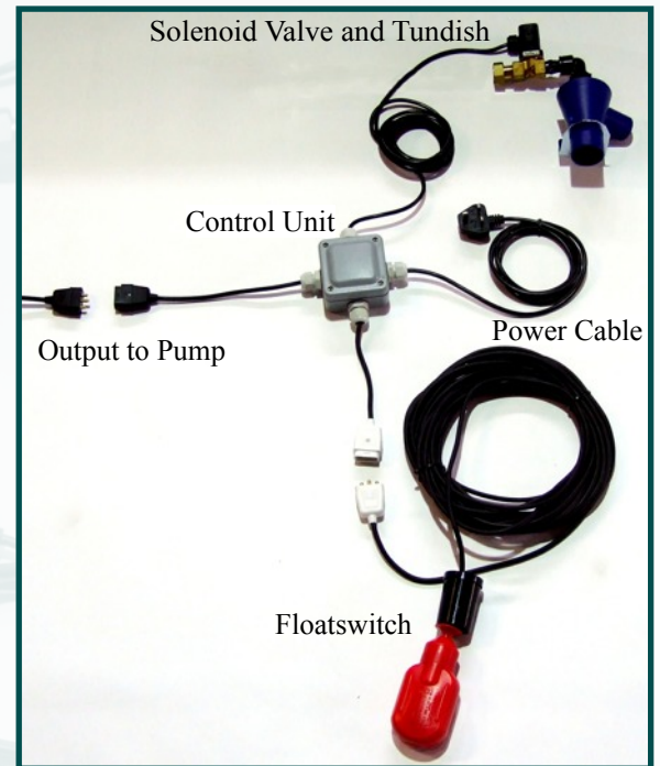
The 3P Rainwater Top-up Switch with Pump Control
